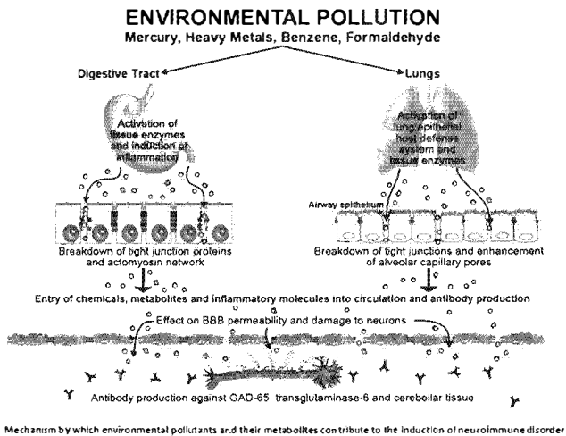
Figure 2. Proposed mechanism for the effect of environmental pollutants on the BBB, leading to neuroautoimmunity. Environmental pollutants enter the system either through inhalation or consumption, activating enzymes and inducing inflammation. This opens the tight junctions, allowing pollutant molecules to enter the circulation, causing autoantibody production. Autoantibodies attack neuronal cells of the CNS, leading to demyelination and neuroautoimmunity.
