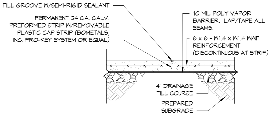
① SLAB CONSTRUCTION JOINT 3/4" = 1'-0"
