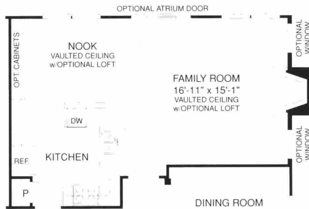
PLAN WITH OPTIONAL SIDE FIREPLACE
